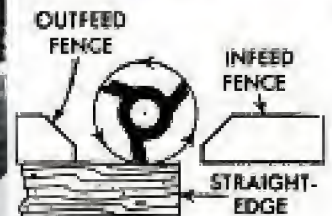
FIRST—SET COMPLETE FENCE EVEN WITH CUTTER
